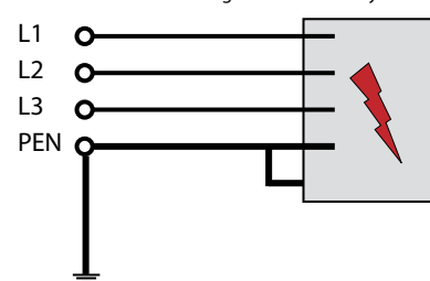
TN-C-System Combined neutral and protective earth conductor to one common conductor throughout the entire system
