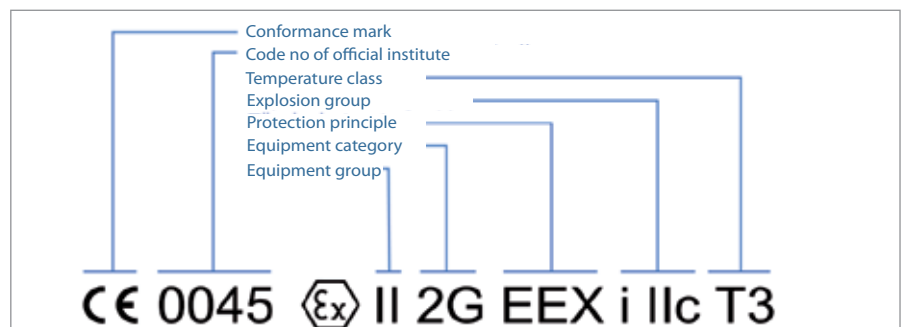
Labelling of devices for operation in potentially explosive atmospheres in accordance with the ATEX product directive (94/9/EC)
